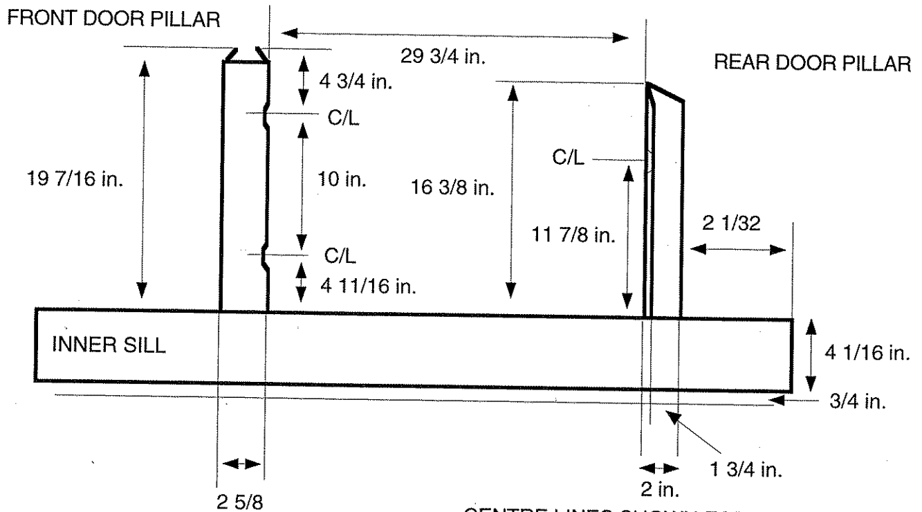
SIDE VIEW OF INNER SILL
