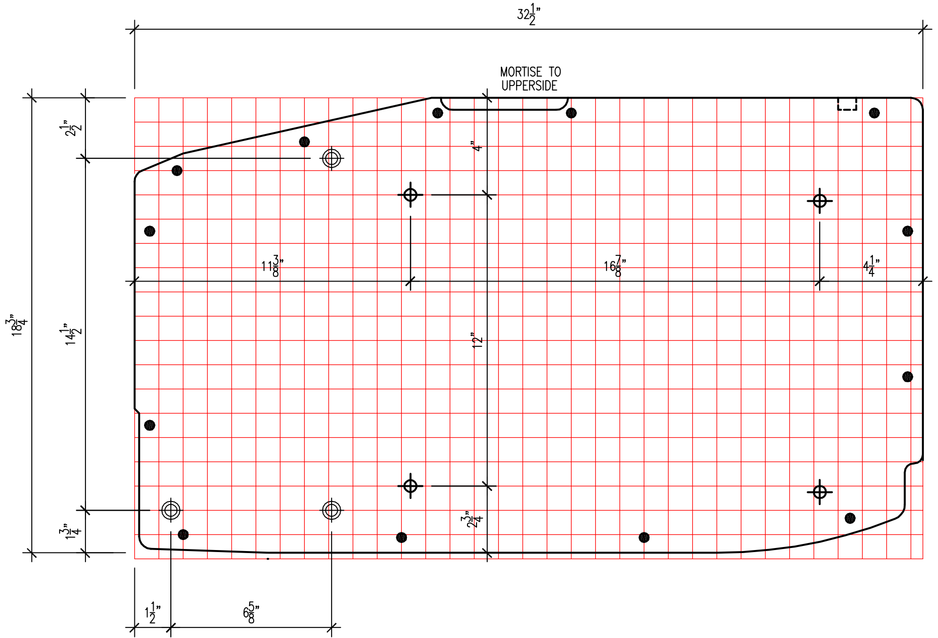
FLOORBOARD-REAR-L.H.
